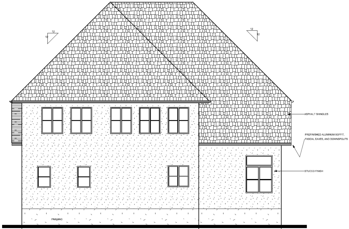
REAR ELEVATION
